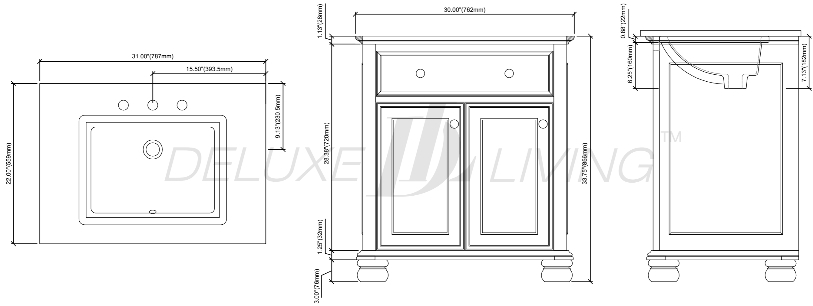
TOP VIEW
